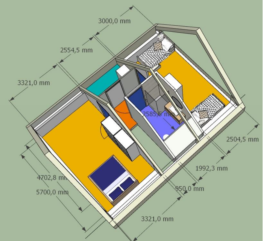
Isometrie verdieping
